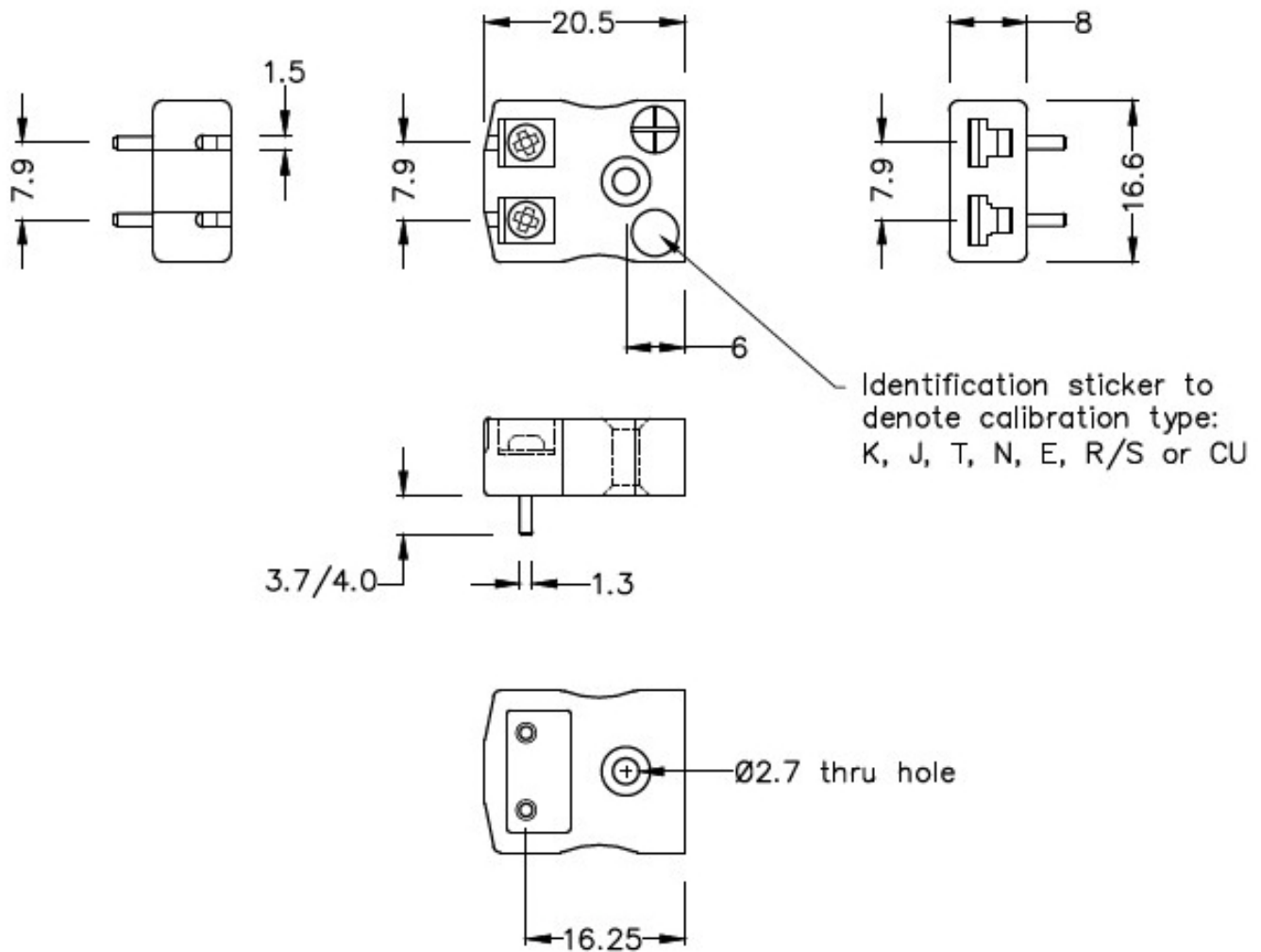
Miniature PCB Socket (dimensions in mm)
