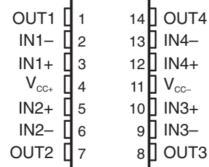
TL974...D, N, OR PW PACKAGE (TOP VIEW)
